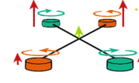
PITCH- AFT
