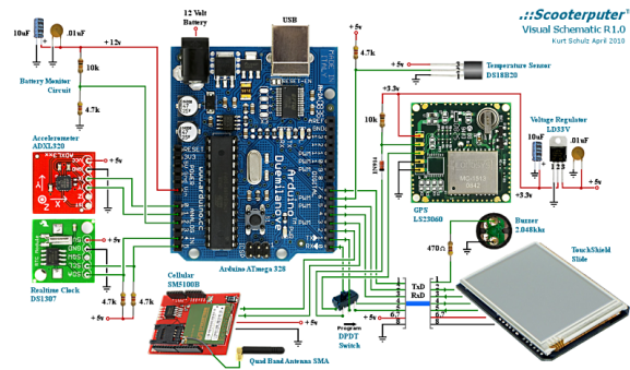
Figure 6. Circuit Diagram
