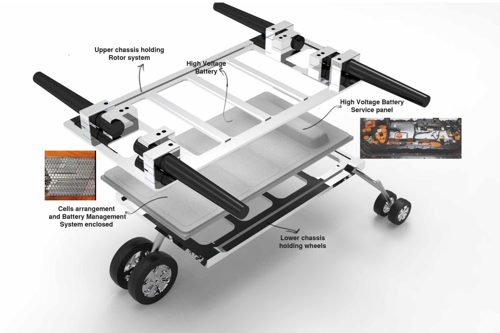
Image 39 : Main chassis design - Expanded view
