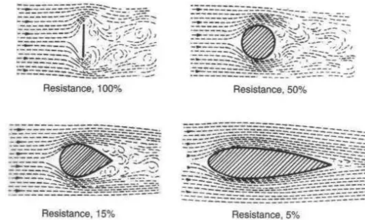
Image 16: Streamlined body and drag resistance
