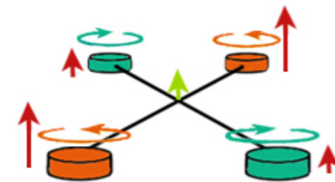
Yaw - Right
