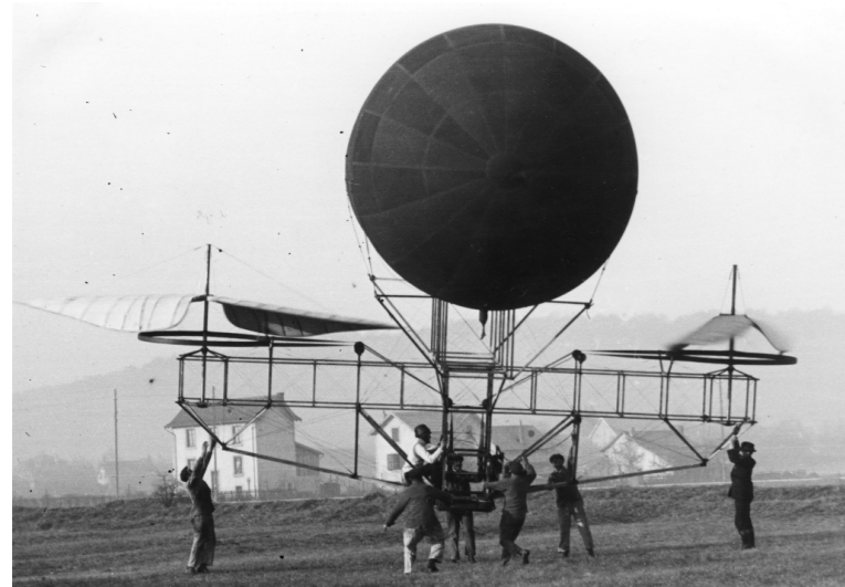
Image 5(a) : Oemichen No.1
