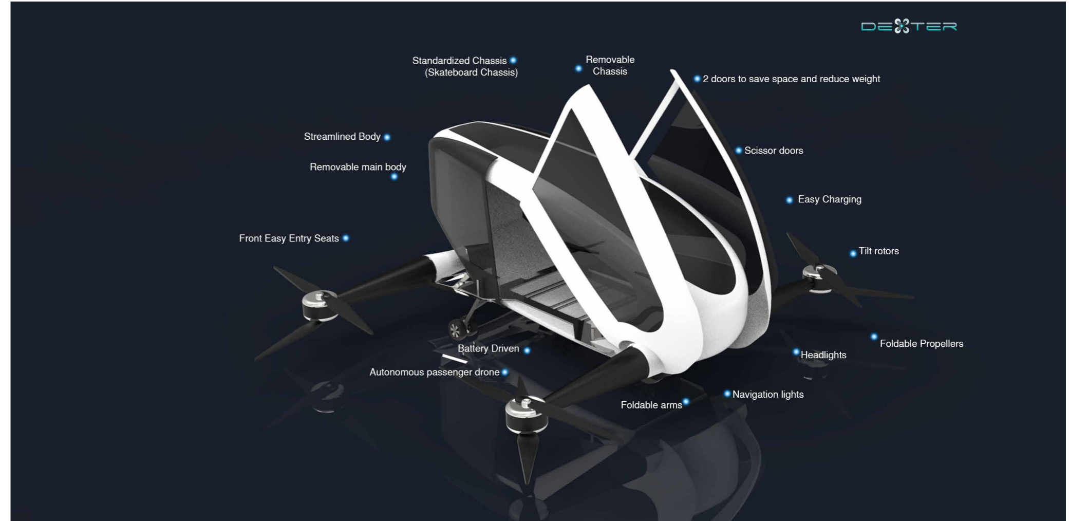
Image 52: Rendered image of Completed model
