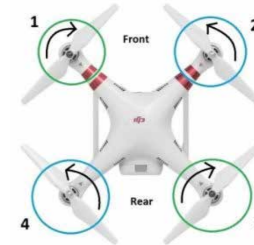
Image 17 Rotational directions on quadcopters
