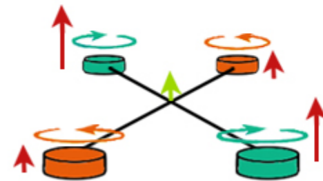
Yaw - Left
