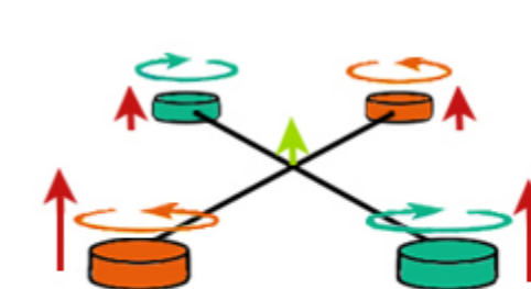
Pitch- Forward
