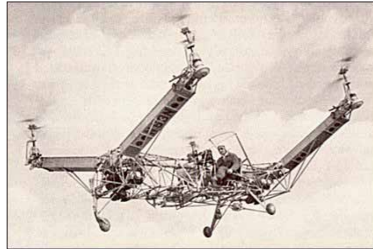
Image 7(b) : Convertawings Model A
