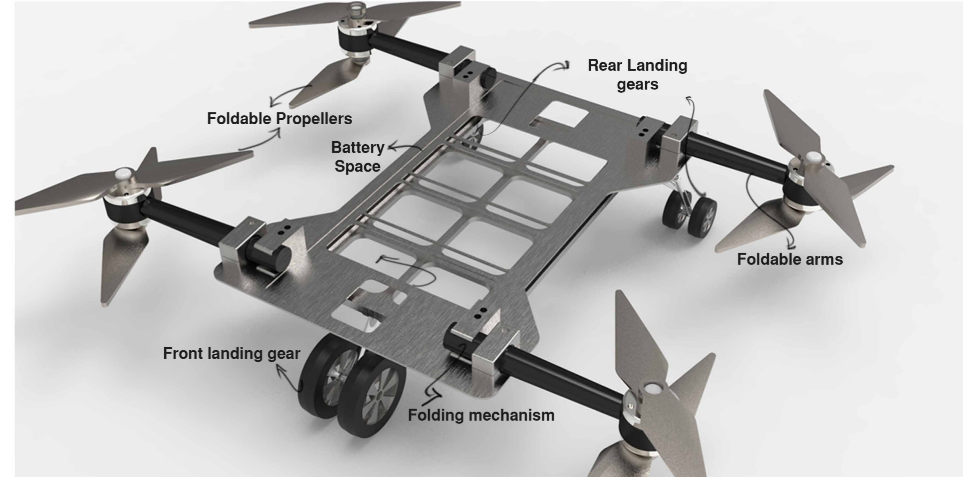
Image 38 : Main chassis design - main parts
