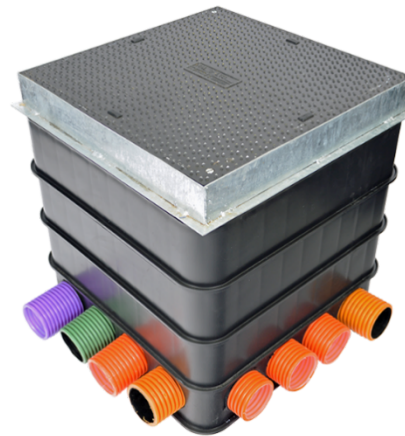
Access chamber
