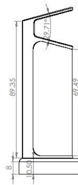
Litter bin
