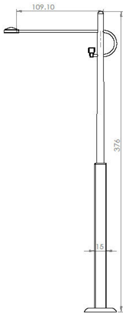
Light pole
