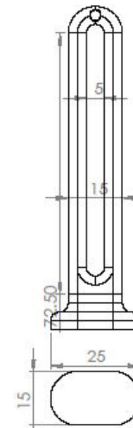
Bollard @ 90 cm distance on the street
