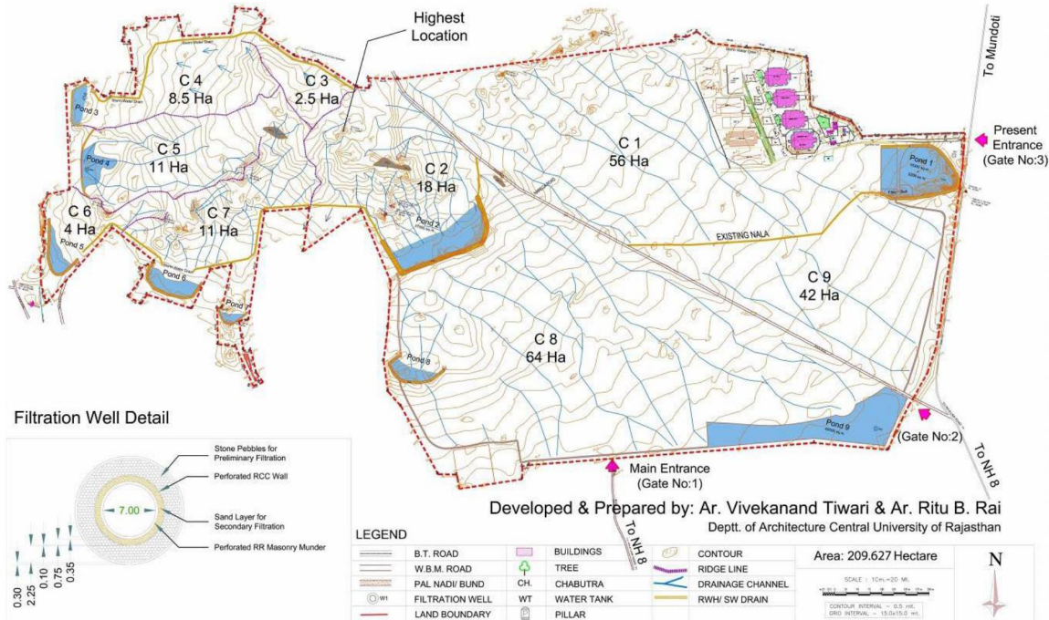
Figure 5: Micro Catchment Drainage Study
